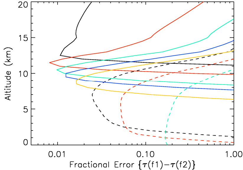
Fig. 3. Simulated fractional error in measuring the difference in optical depth for selected pairs of frequencies as a function of altitude. The background atmosphere is the Lowtran 2 mid-latitude summer profile. Fractional errors take into account expected measurement uncertainty, atmospheric absorption and defocusing, and the effects of turbulent variations in both dry and wet real refractivity. Solid lines are 183 GHz pairs (Black: 183.0, 179.0 GHz; Red: 181.7, 179.0 GHz; Green: 180.0, 176.0 GHz; Blue: 179.0, 165.0 GHz; Orange: 176.0, 165.0 GHz) and dashed lines for 22 GHz pairs (Black: 22.0, 20.0; Red: 21.0, 18.0 GHz; Green: 19.0, 16.0 GHz).
