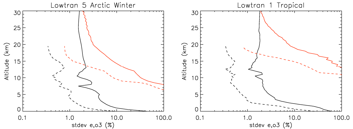
Fig. 5. Standard deviation of simulated errors of water vapor (black) and ozone (red) from satellite (solid) and aircraft occultations (dashed). Panel a is for arctic winter conditions and Panel b is for tropical conditions.
