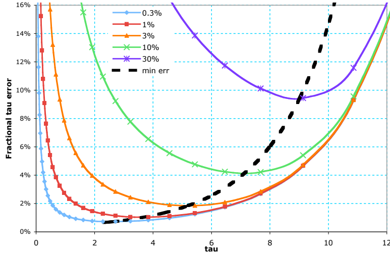
Fig. 2. The fractional error in measured \Delta\tau_{12} versus \tau_1 for turbulence-induced, amplitude ratio errors (after amplitude ratioing) ranging from 0.3% to 30%, for S_{v10} = S_{v20} = 2000 , a_{12} = 0.2 , 200 m vertical resolution and V_0 = 2.5 km/sec. The black dashed line defines the curve of minimum fractional \Delta\tau_{12} error
