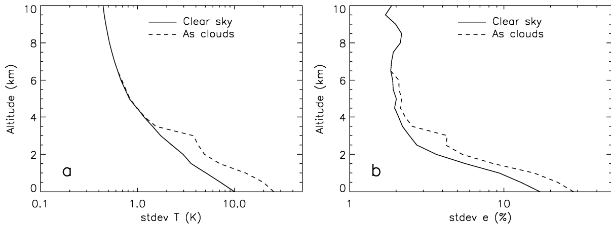
Fig. 4. Computed standard deviation of the errors in the retrievals of (a) temperature and (b) water vapor pressure using simulated ATOMMS observations. The background atmosphere is the Lowtran 2 mid-latitude summer profile. Solid lines are for clear sky conditions, while the dashed lines were computed after placing two broken decks of altostratus clouds between 3 - 3.5 and 6 - 6.5 km altitude with liquid water contents of 0.3 and 0.2 \text{gm}^{-3} respectively. The cloud fields are highly non-symmetric about the local tangent point.
